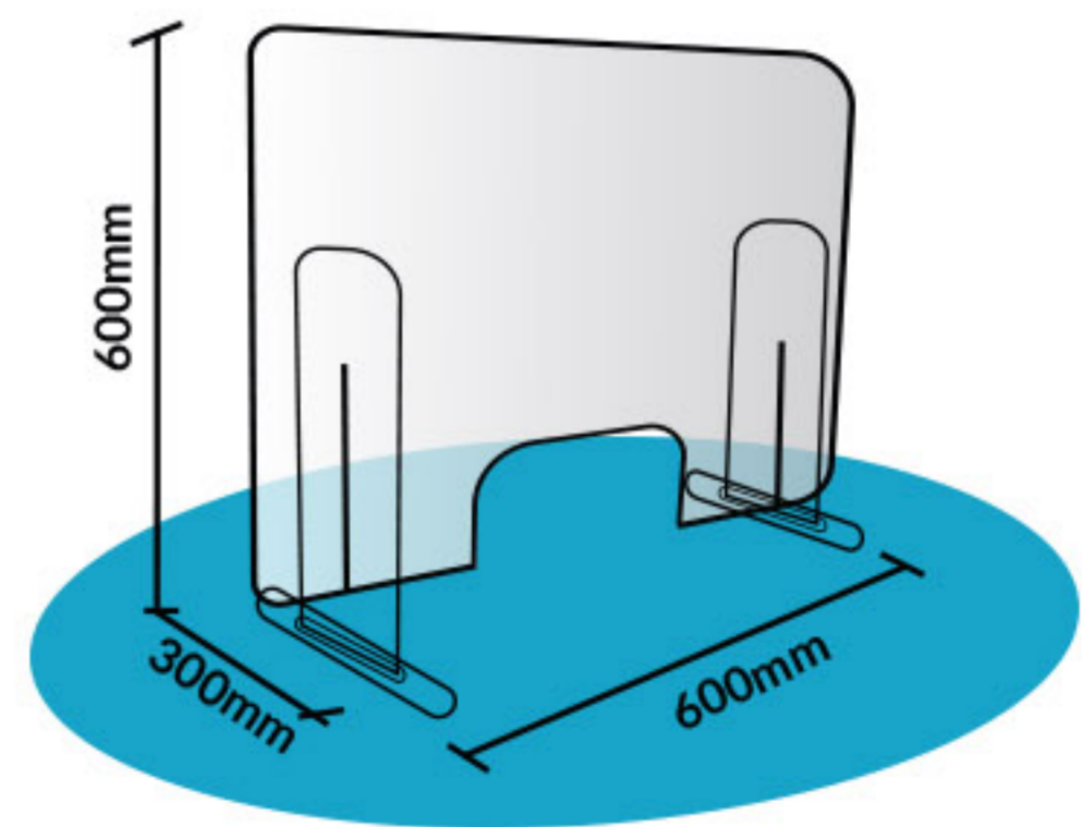
SMALL SCREEN/CUT-OUT AREA
