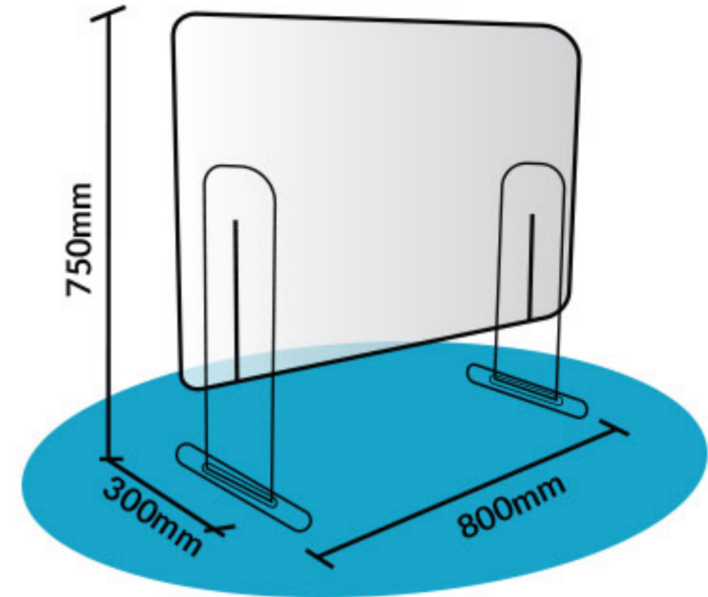
3/4 SCREEN WITH ACCESS
